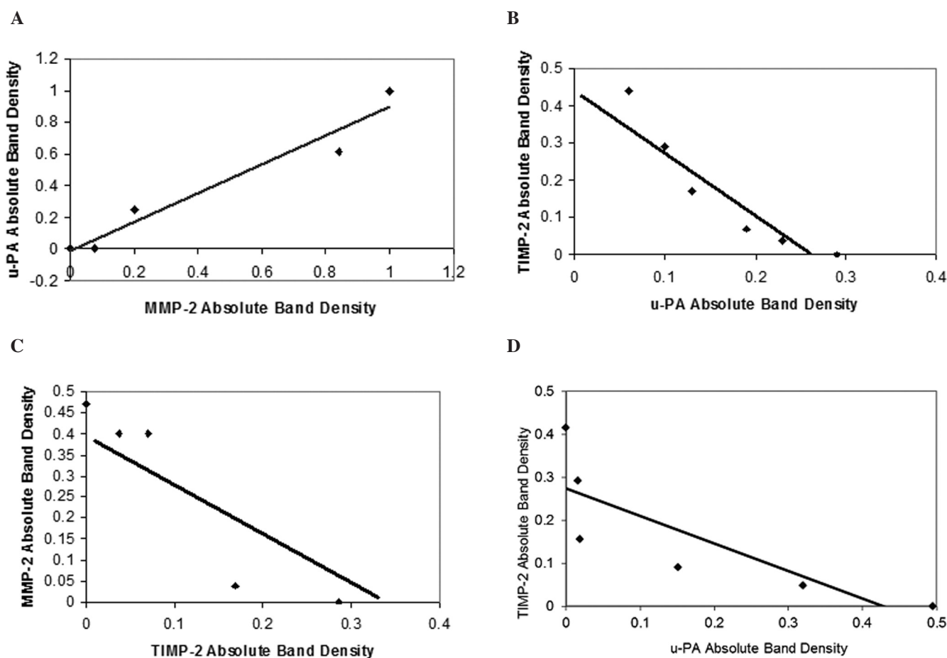
Figure 4. (A) Correlation between the effects of NM on prostate cancer PC-3 u-PA and MMP-2 expression. (B) Correlation between the effects of NM on prostate cancer PC-3 TIMP-2 and u-PA expression. (C) Correlation between the effects of NM on prostate cancer PC-3 MMP-2 and TIMP-2 expression. (D) Correlation between the effects of NM on prostate cancer DU-145 u-PA and TIMP-2 expression.
